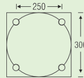
Mounting Dimension
